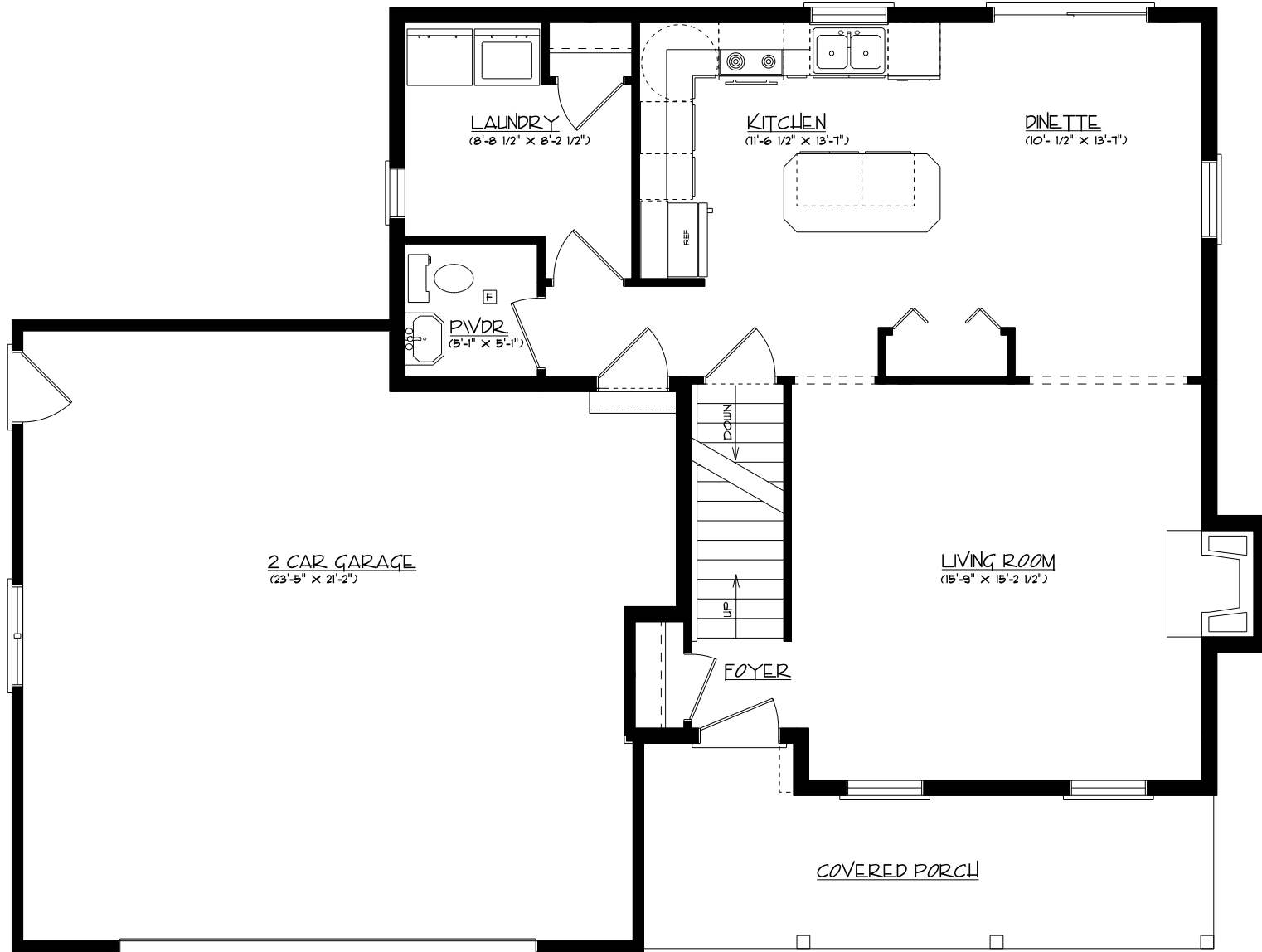
FIRST FLOOR PLAN 716 SQ. FT.
